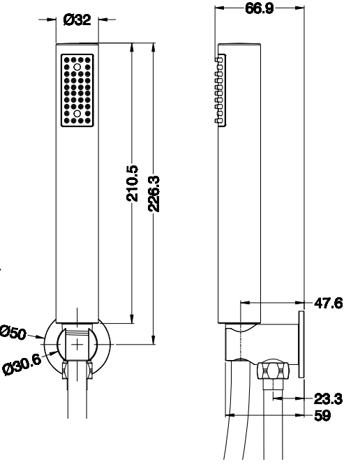
Round Outlet Holder with Hose and Handset RDS001
