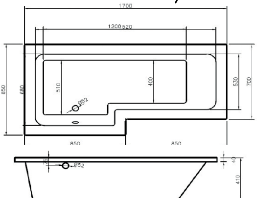
Right Hand L Shaped Bath
