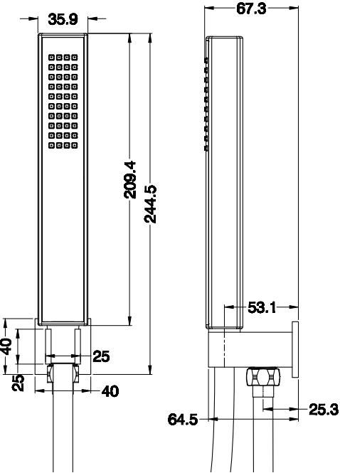
Square Outlet Holder with Hose and Handset HDS001
