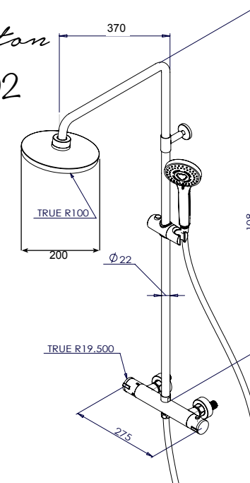
SAS Thermostatic Shower SK008
