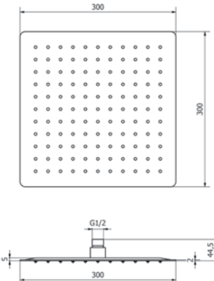
Stainless Steel 300mm Square Head SSSQH30
