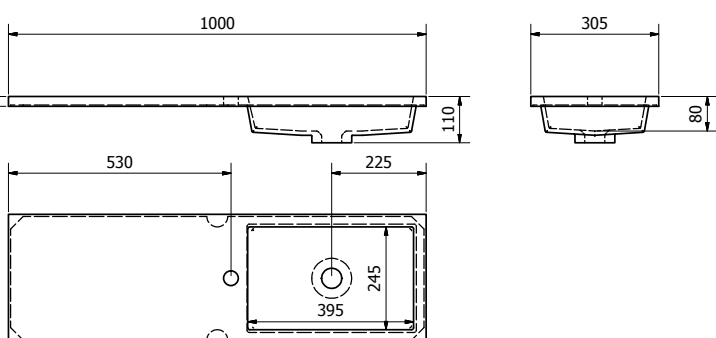
Slimline Counter Top Basin
