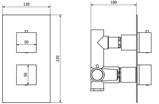
Square Concealed Valve TSCV01
