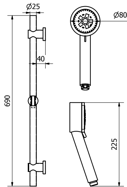
Elite Shower SK005
