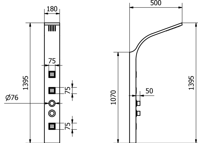
Thermostatic Shower Panels BSP001 / WSP002
