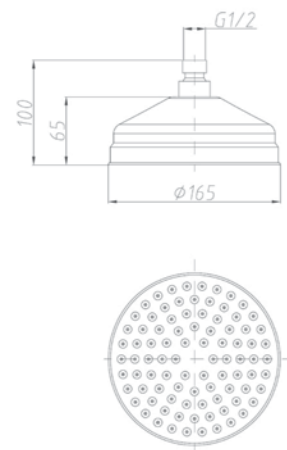
7" Traditional Head TRH07
