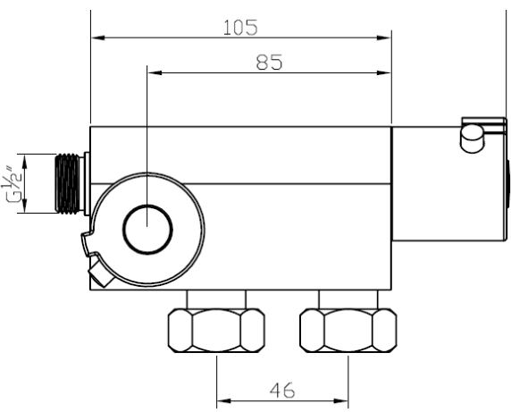
Vertical Thermostatic Bar Valve VTBV01
