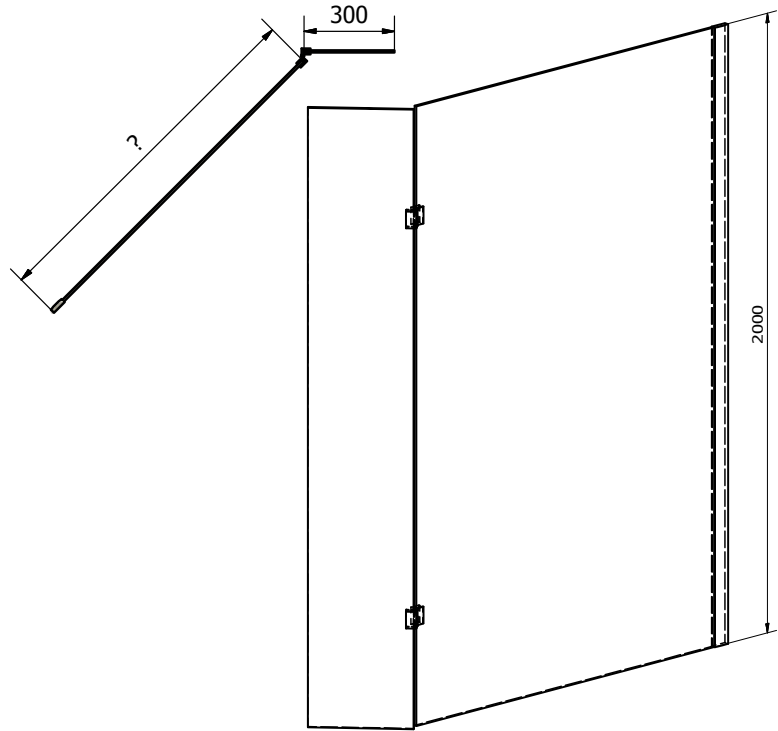
4 Fold Bath Screen CEFO01
