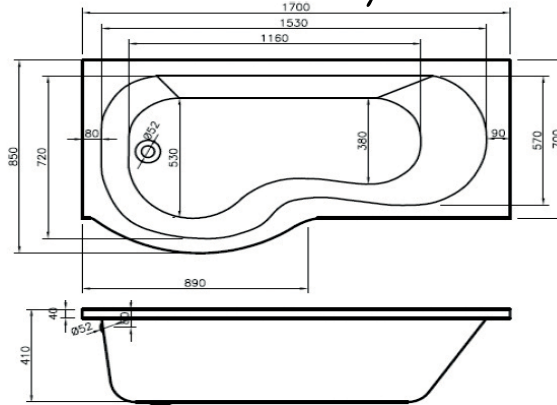
Right Hand D Shaped Bath
