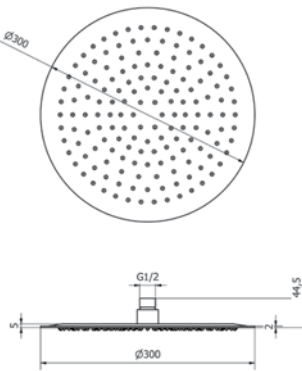
Stainless Steel 300mm Round Head SSRDH30
