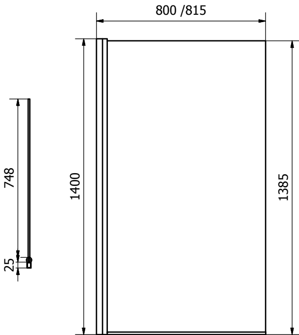
Square Bath Screen CEL002
