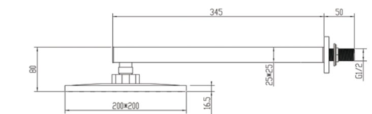
Square Arm / Head SQARM / SQH22
