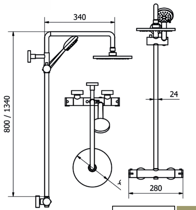
Thermostatic Shower SK006
