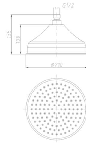
8" Traditional Head TRH08
