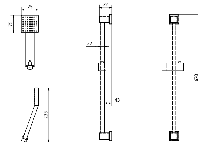
Square Slide Rail Kit SSRK01
