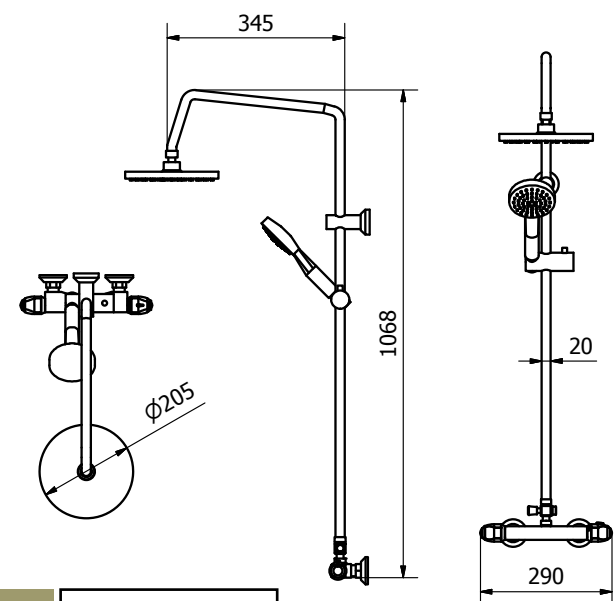
Thermostatic Shower SK007
