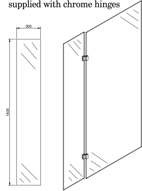
CS030 Wet Room Panel Hinged
