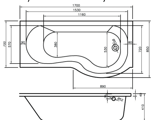
Right Hand D Shaped Bath
