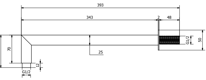
Wall Mounted Round Shower Arm ARMRD
