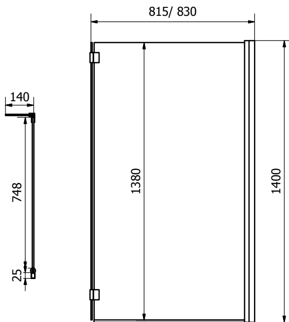
Bath Screen with Flipper Panel CEL004
