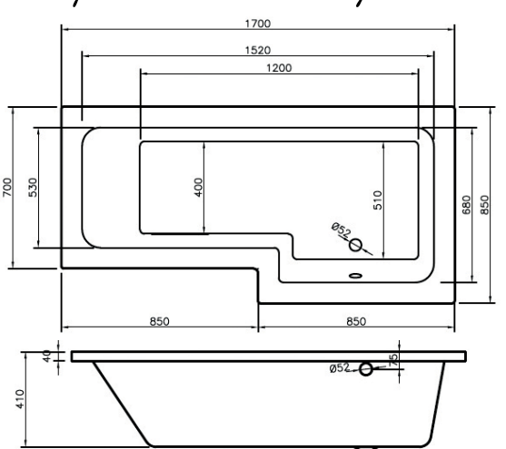
Right Hand L Shaped Bath
