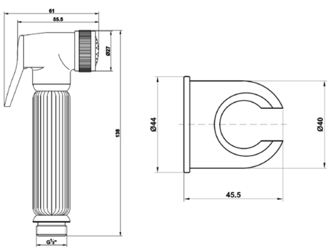
Douche Brass Shower Spray Kit with Wall Bracket and Hose DOU002
