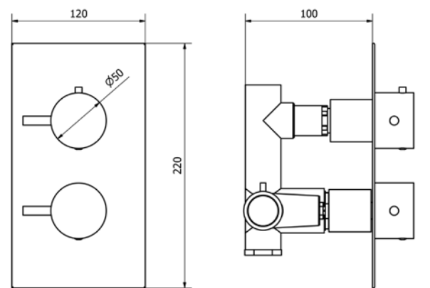
Square Concealed Valve TSCV01
