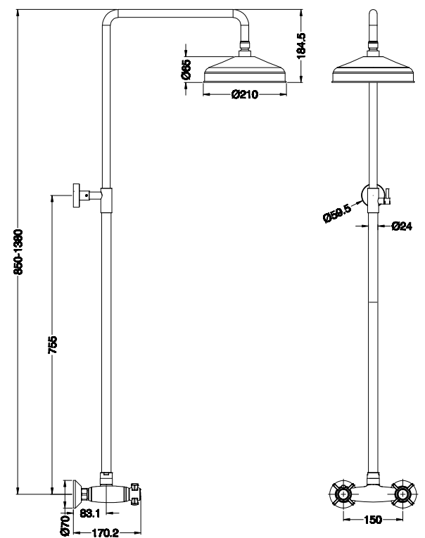
Round Concealed Valve TRCV02
