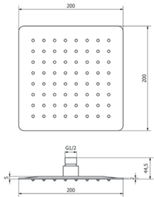
Stainless Steel 200mm Square Head SSSQH20
