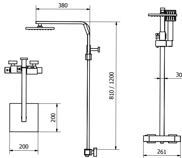
Thermostatic Shower SK007
