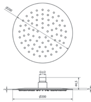
Stainless Steel 200mm Round Head SSRDH20
