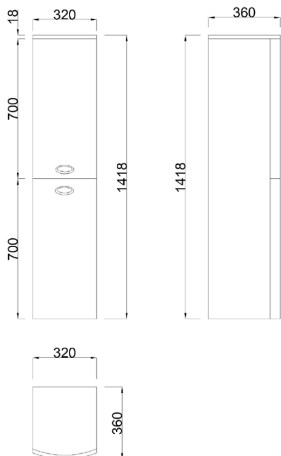
Tall Wall Mounted Cabinet TWMC01-GW
