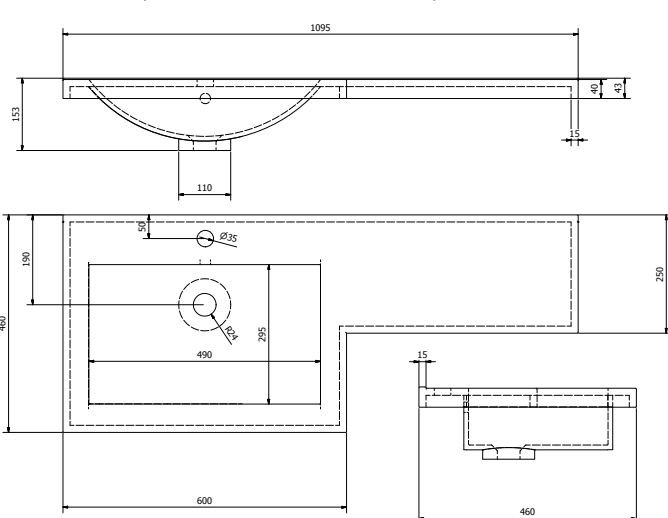
L Shaped Counter Top Basin
