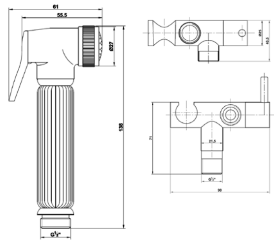
Douche Brass Shower Spray Kit with Shut Off Valve and Hose DOU001
