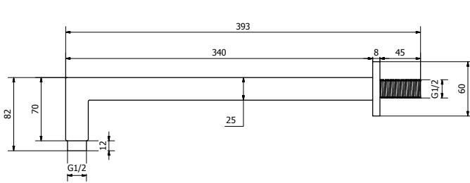
Wall Mounted Square Shower Arm ARMSQ
