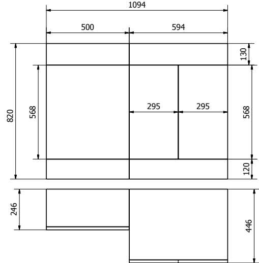
L Shaped Furniture
