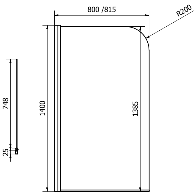
Curved Top Bath Screen CEL001
