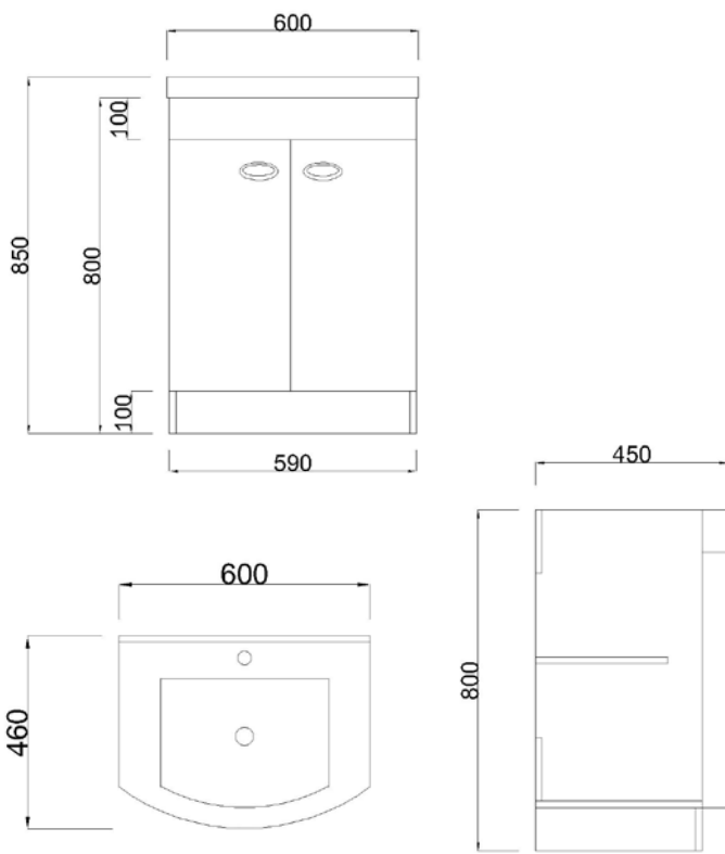
Eye D-shaped Basin Unit with Basin BU001-UNIT-BASIN-RF
